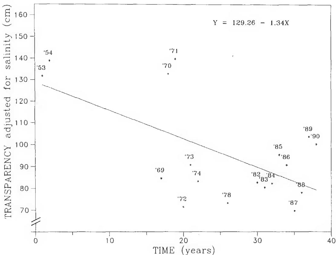
Figure 7. Annual mean Secchi disk transparency from 1953 through 1990 adjusted for salinity.
